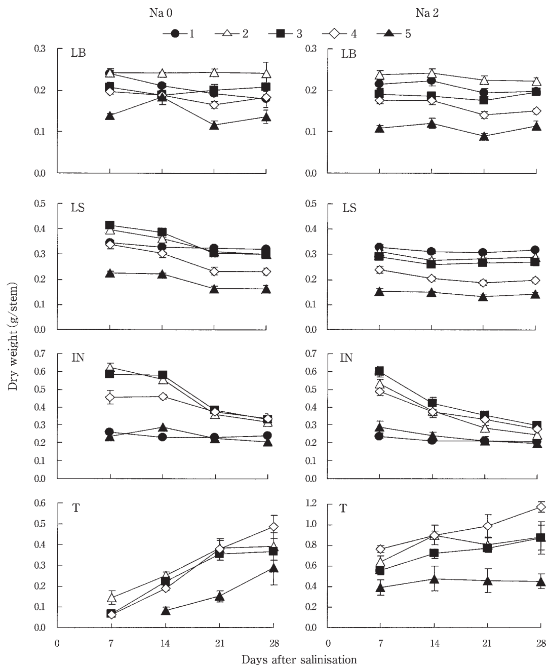
Fig. 3 Changes in dry weight after salinisation with 100 mM NaCl.
