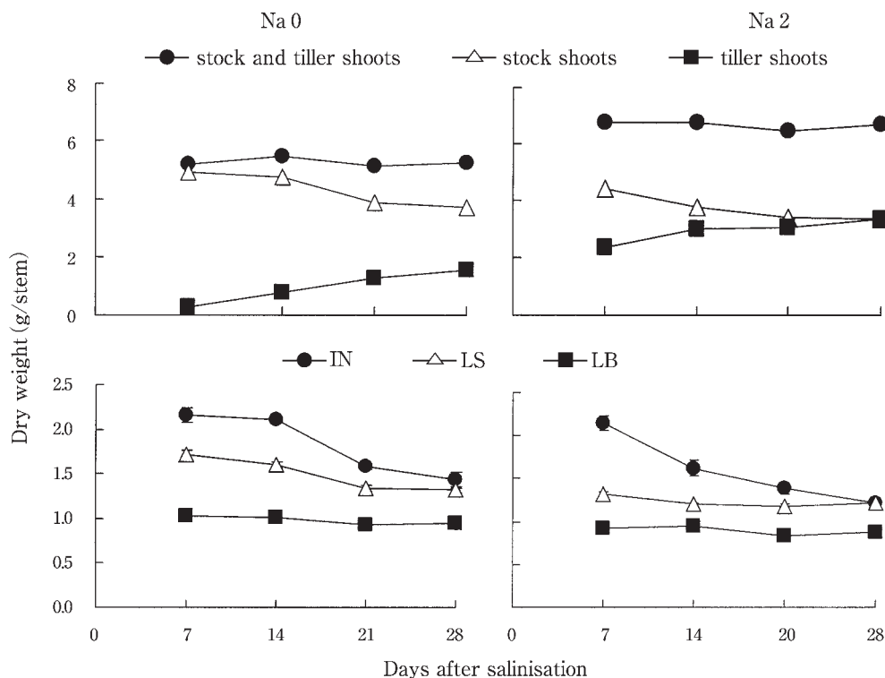
Fig. 2 Changes in dry weight after salinisation with 100 mM NaCl.
