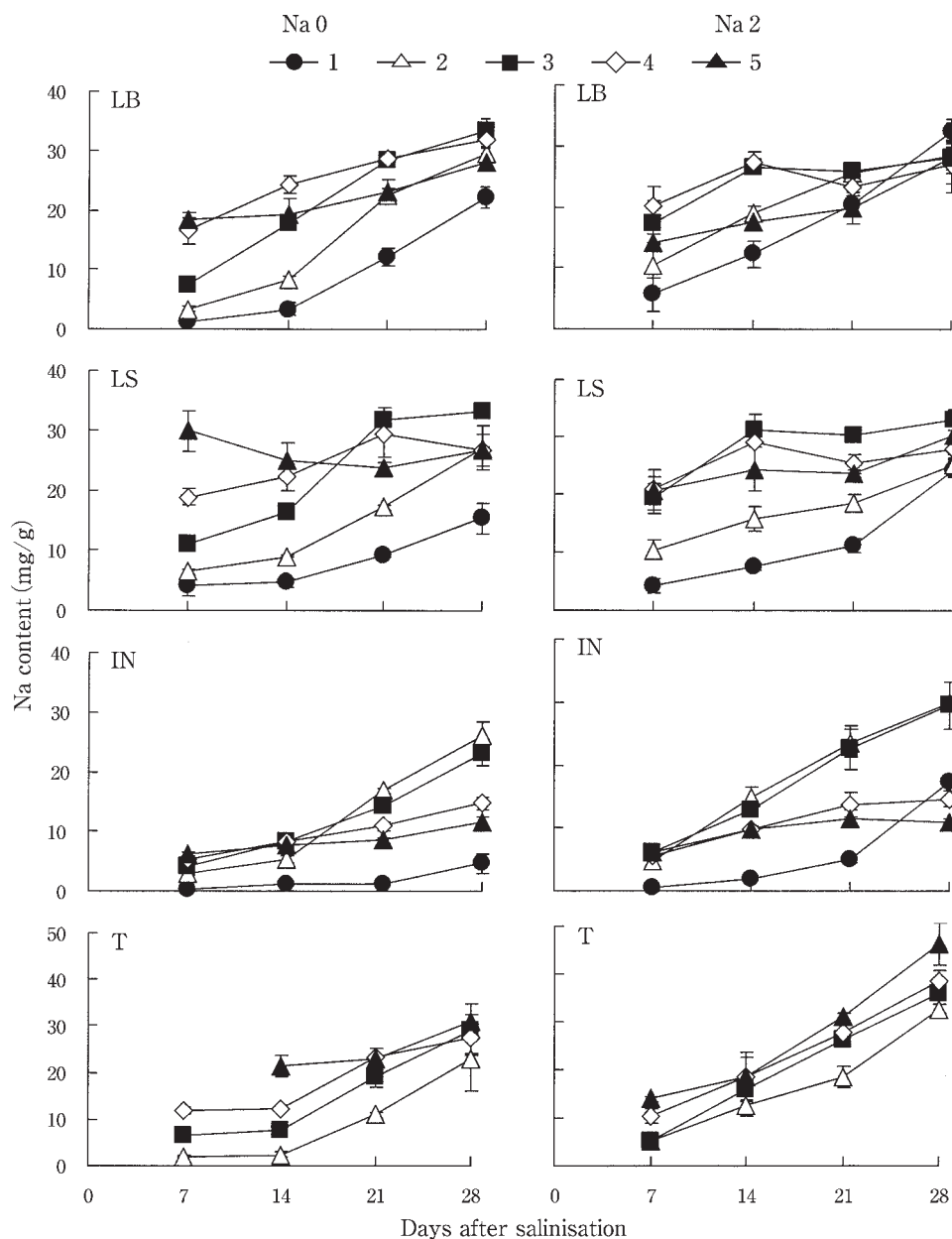
Fig. 4 Changes in sodium contents after salinisation with 100mM NaCl.
